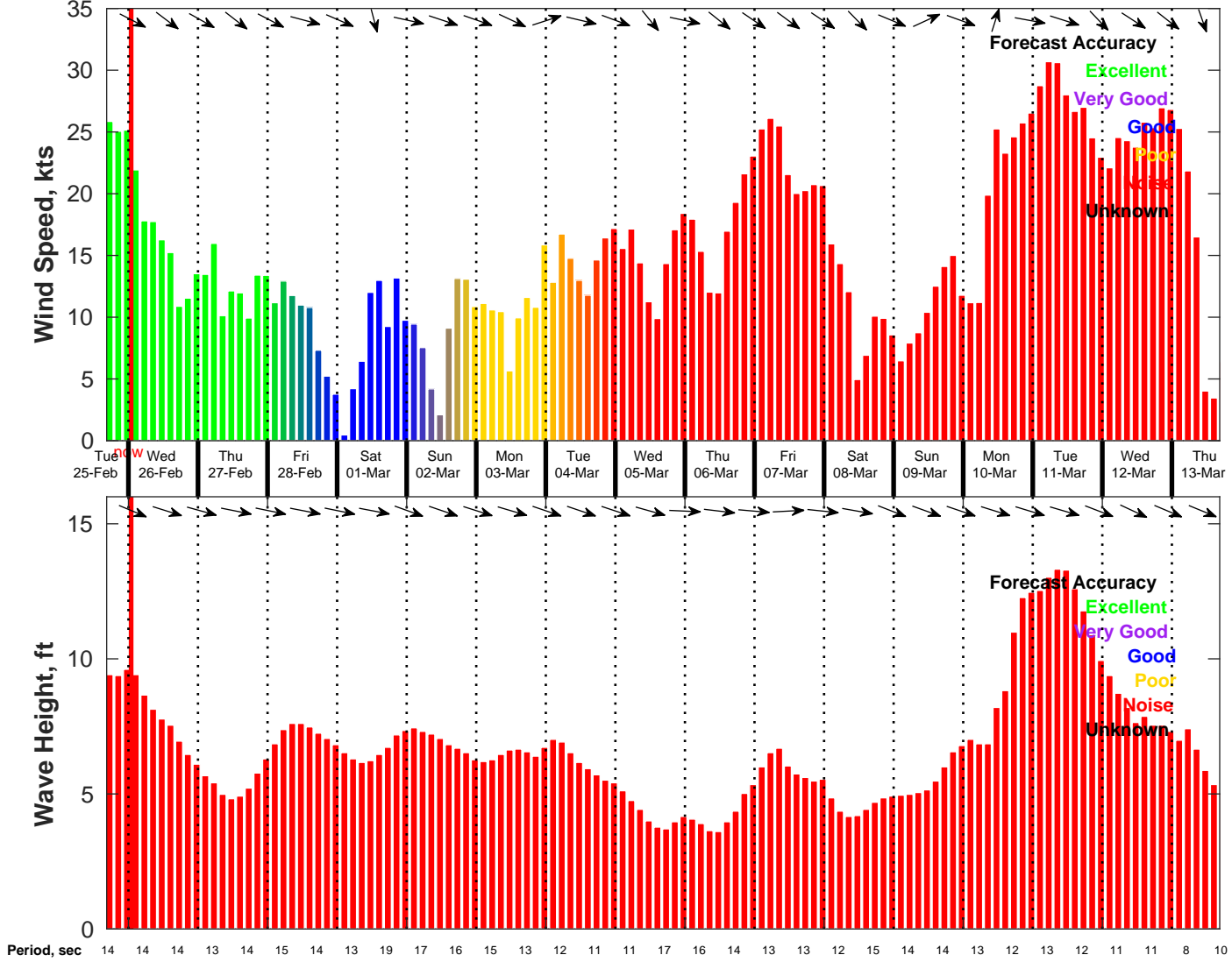
Wind & Wave Forecast for NDBC 46069 from 25-Feb-2025 16:00:00 to 13-Mar-2025 16:00:00
