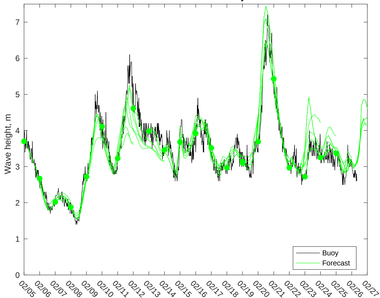
NDBC 46246 vs CMEMS Waves: 0 to 3 day forecast
