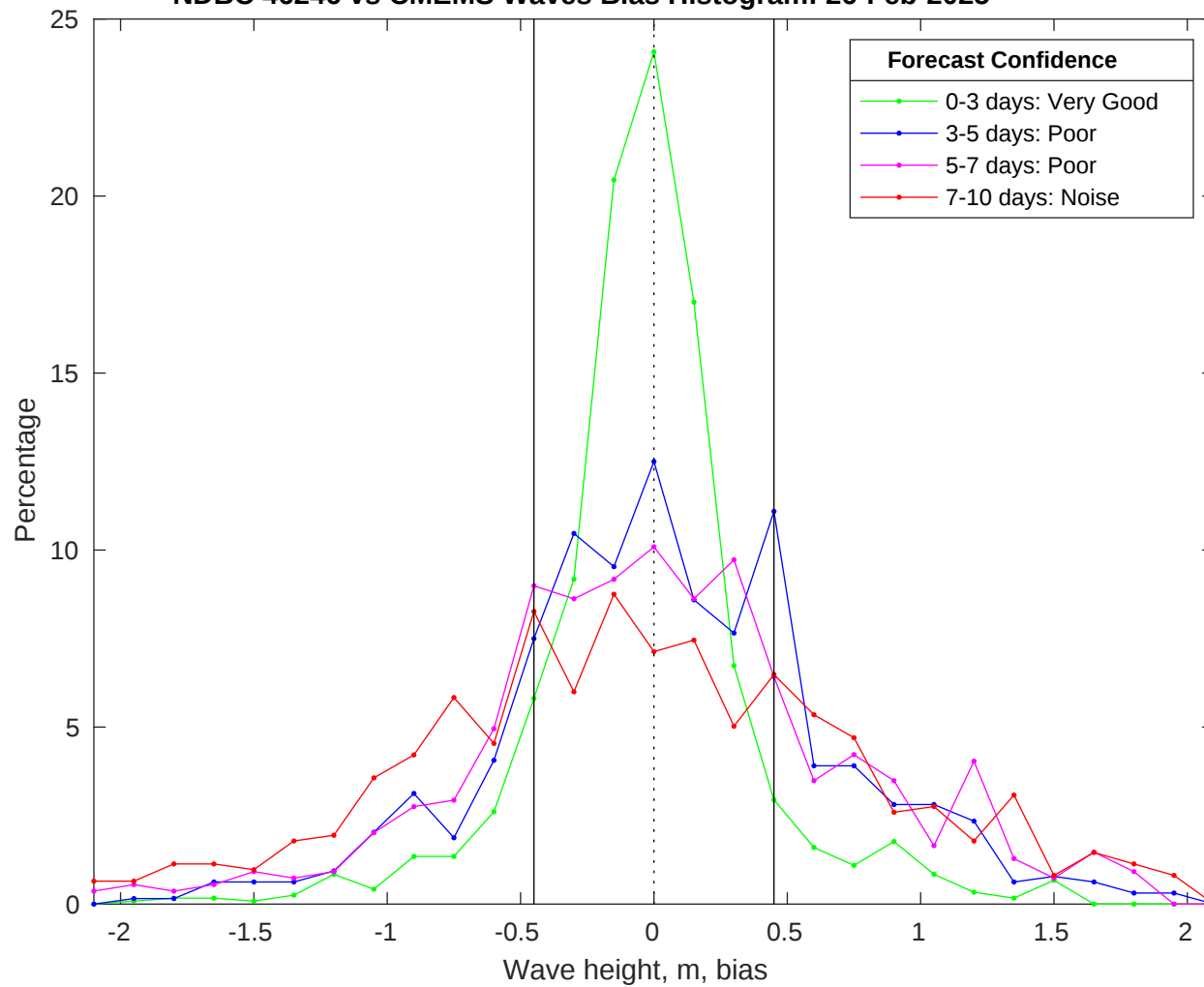
NDBC 46246 vs CMEMS Waves Bias Histogram: 26-Feb-2025
