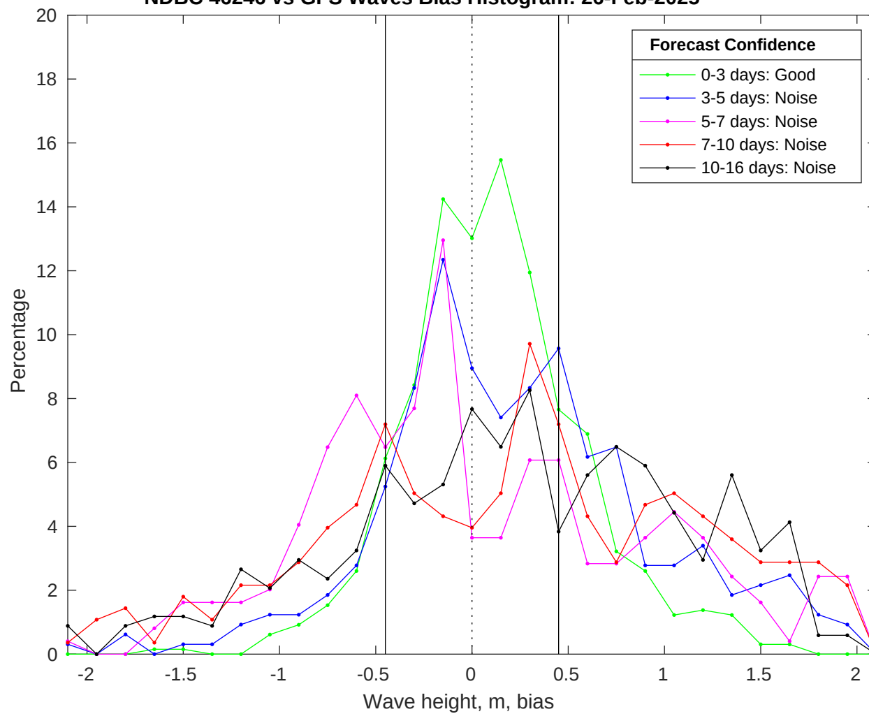
NDBC 46246 vs GFS Waves Bias Histogram: 26-Feb-2025
