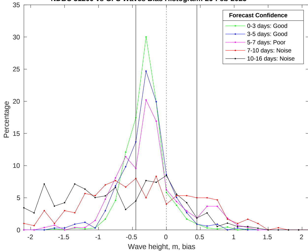
NDBC 51209 vs GFS Waves Bias Histogram: 26-Feb-2025
