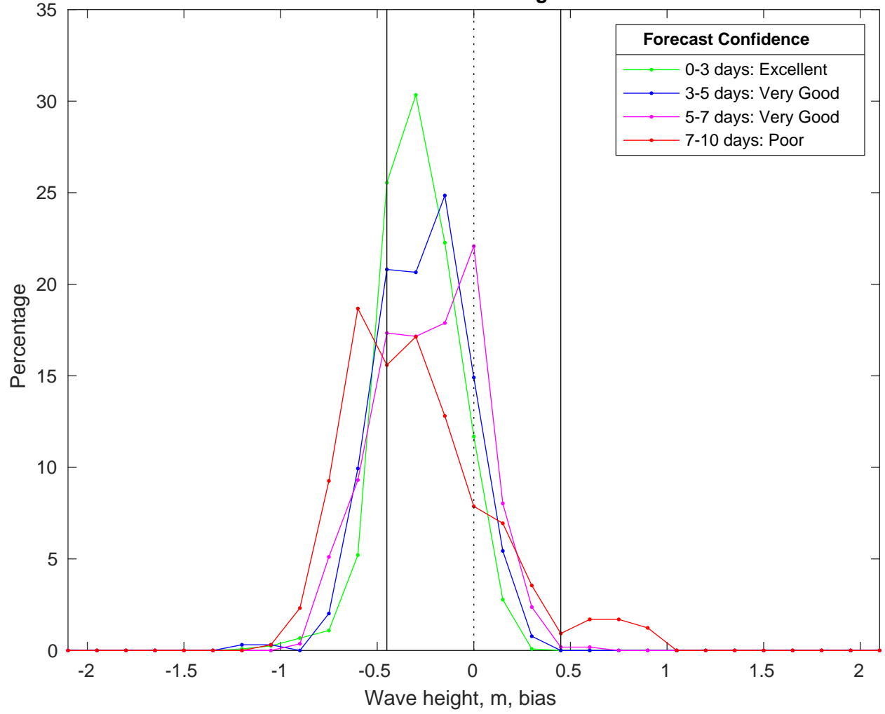
NDBC 52211 vs CMEMS Waves Bias Histogram: 26-Feb-2025
