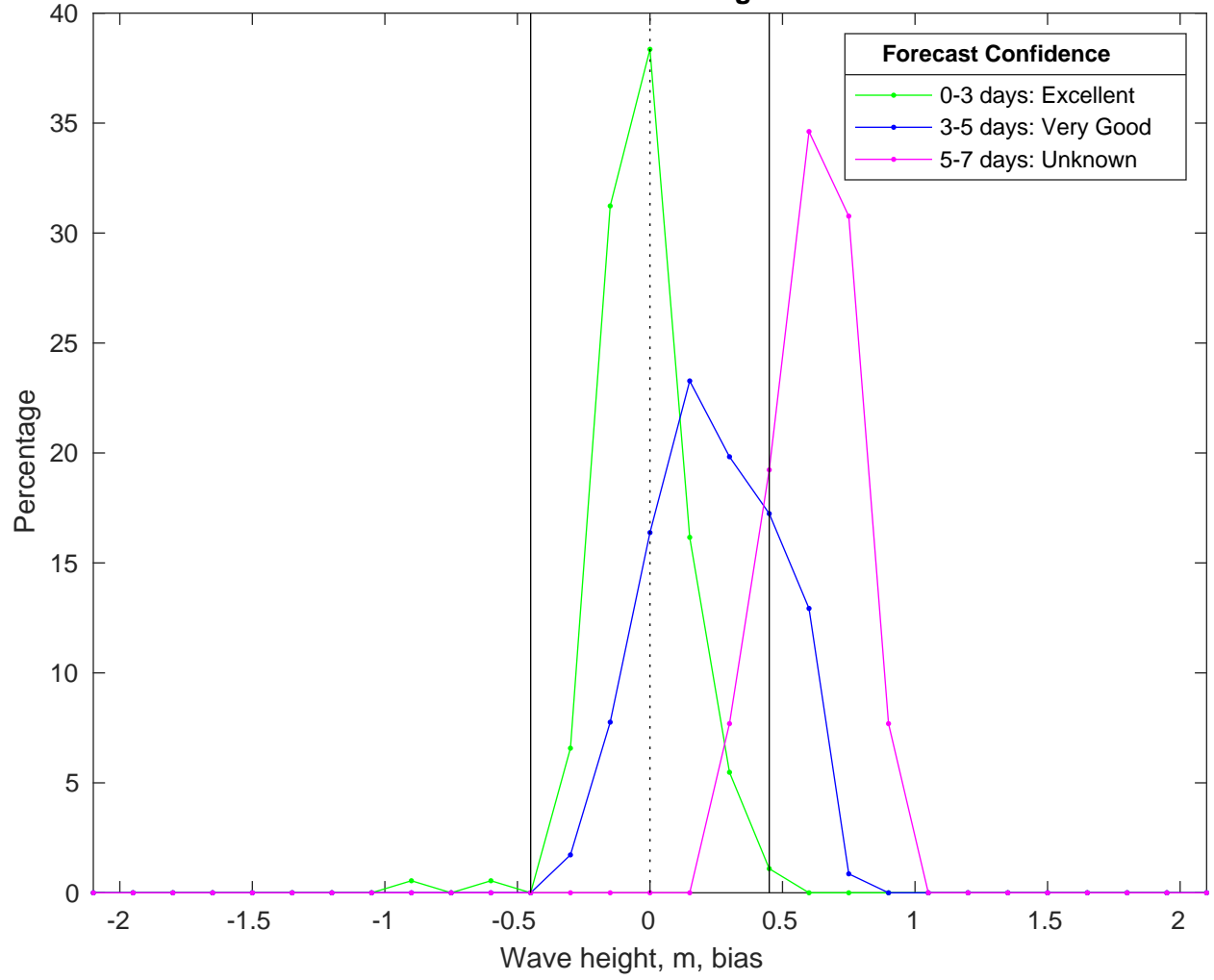
NDBC 52212 vs CMEMS Waves Bias Histogram: 26-Feb-2025
