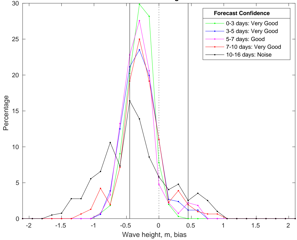
NDBC 52212 vs GFS Waves Bias Histogram: 26-Feb-2025
