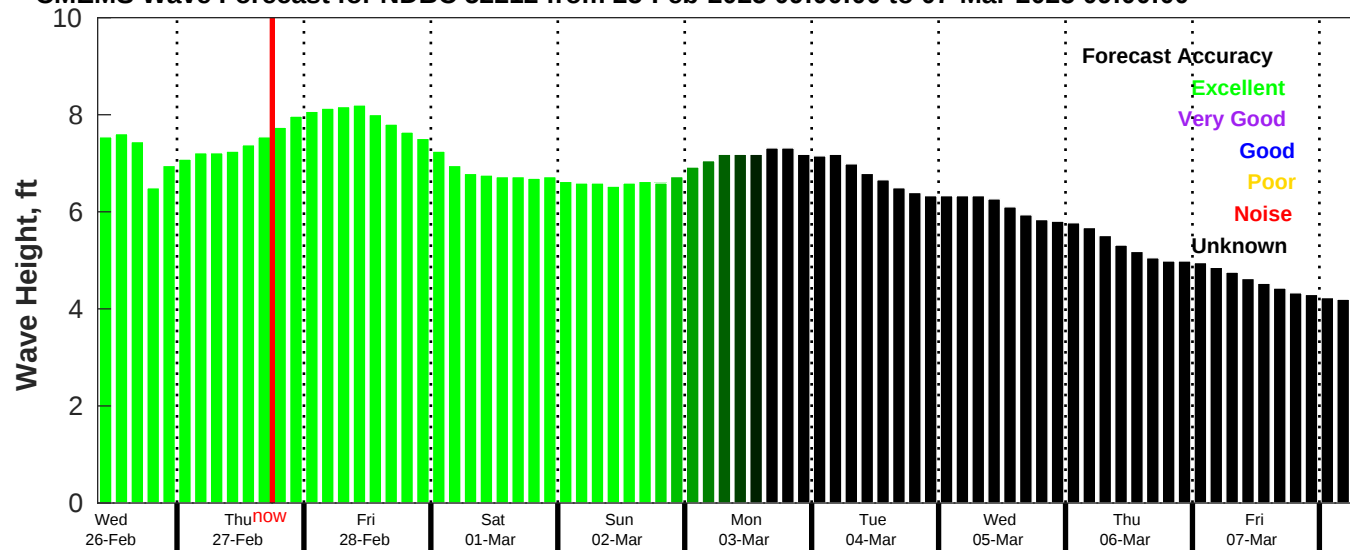
CMEMS Wave Forecast for NDBC 52212 from 25-Feb-2025 09:00:00 to 07-Mar-2025 09:00:00
