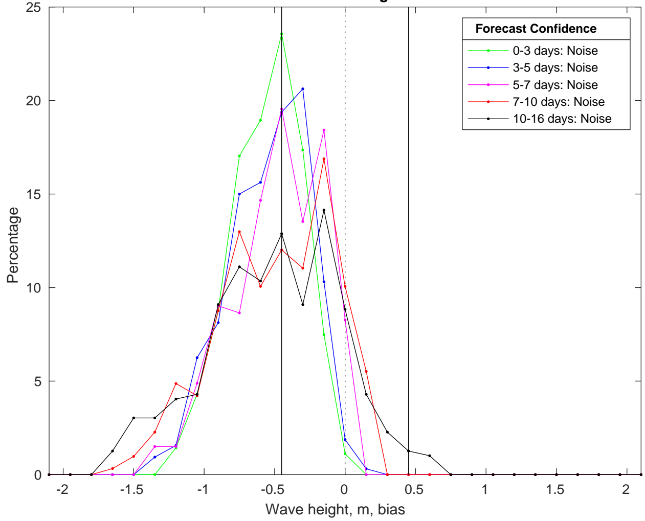
NDBC 52213 vs GFS Waves Bias Histogram: 26-Feb-2025
