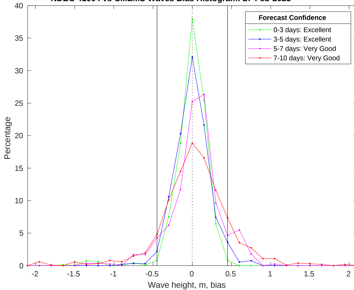
NDBC 41004 vs CMEMS Waves Bias Histogram: 27-Feb-2025
