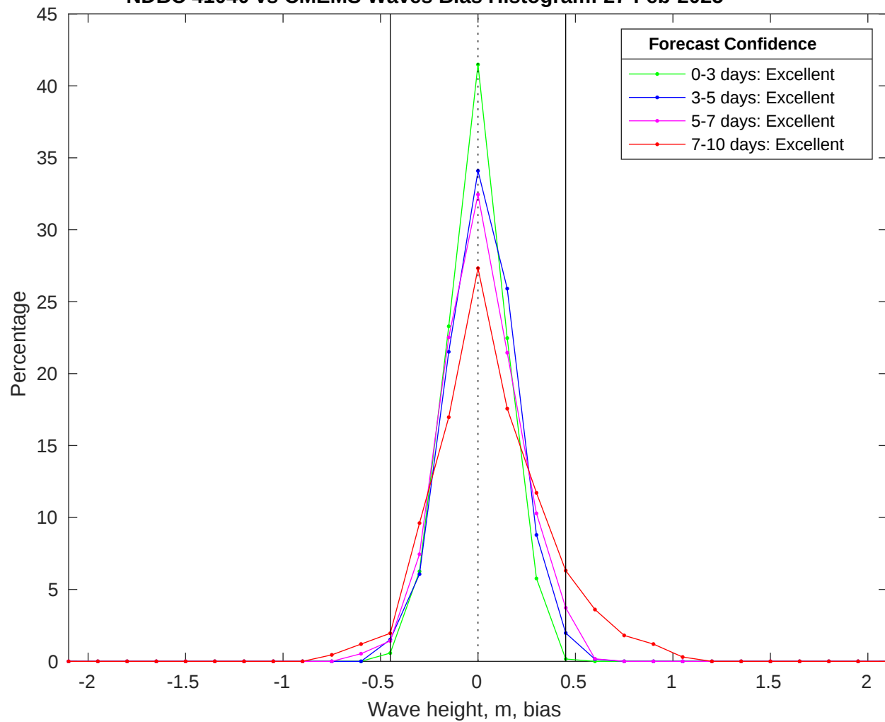
NDBC 41040 vs CMEMS Waves Bias Histogram: 27-Feb-2025
