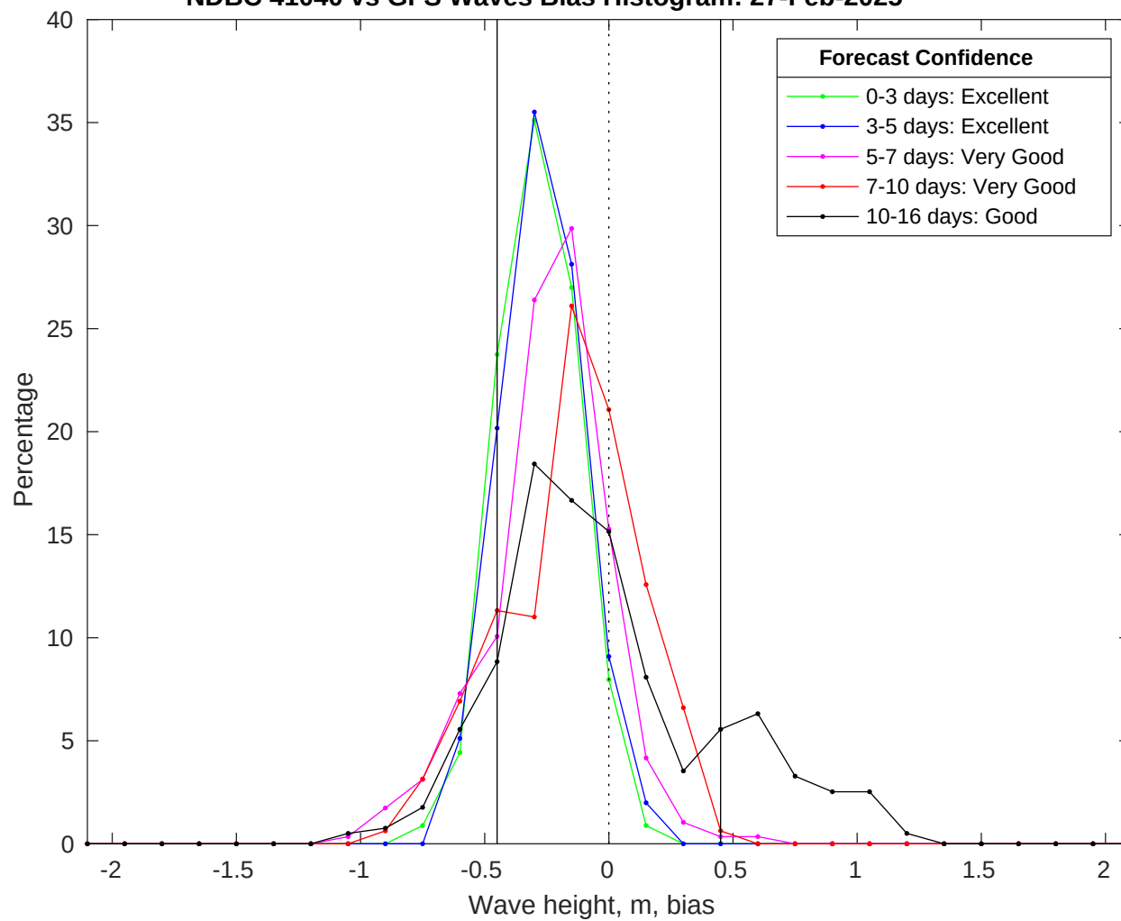
NDBC 41040 vs GFS Waves Bias Histogram: 27-Feb-2025
