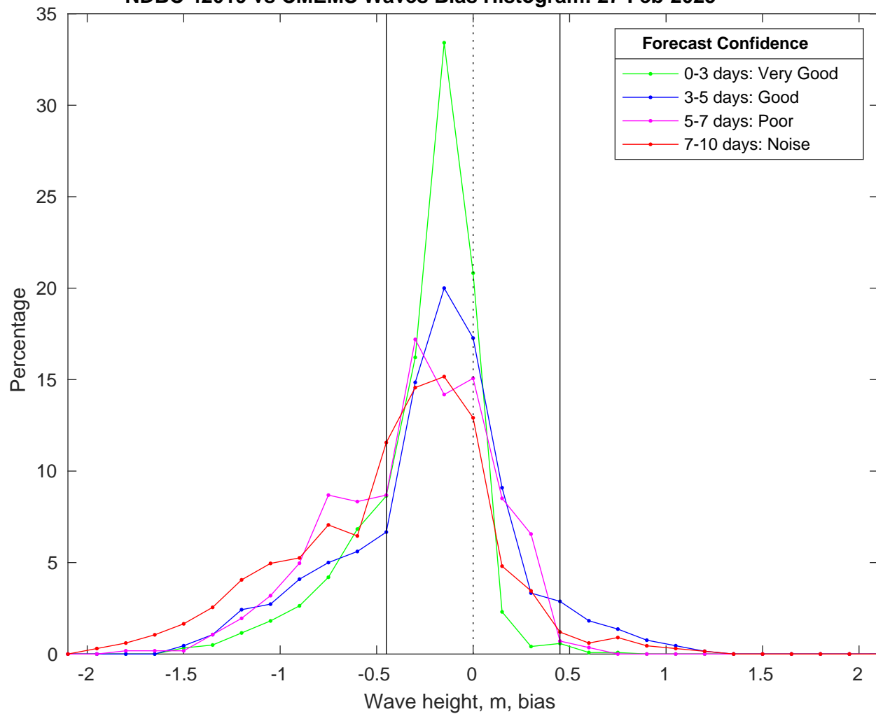
NDBC 42019 vs CMEMS Waves Bias Histogram: 27-Feb-2025
