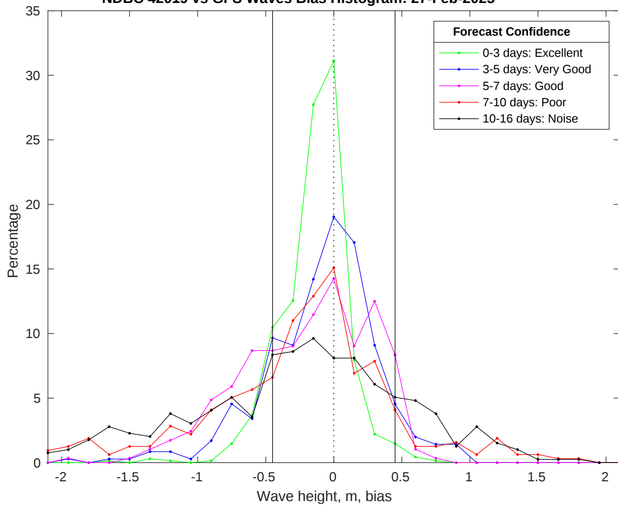
NDBC 42019 vs GFS Waves Bias Histogram: 27-Feb-2025
