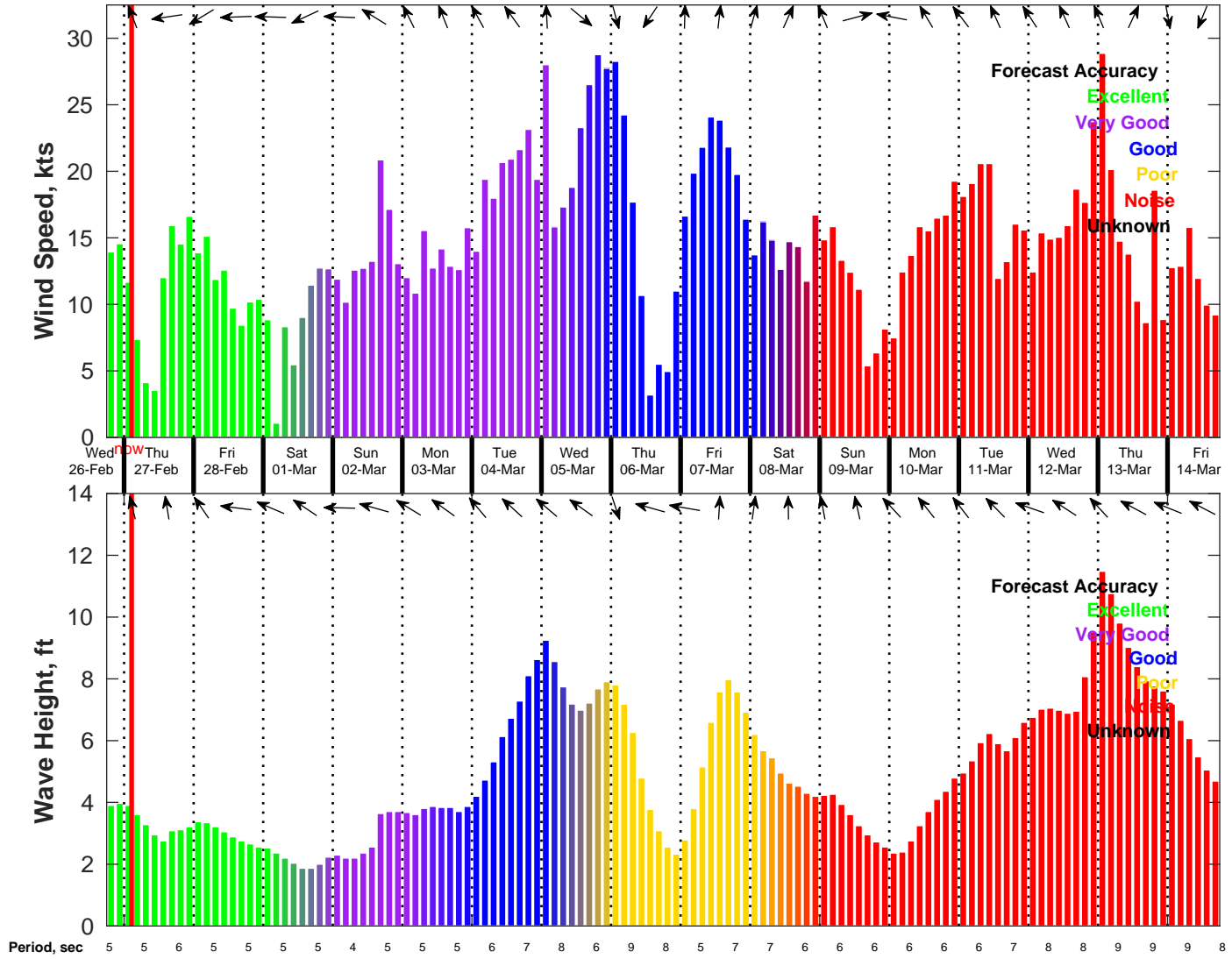
Wind & Wave Forecast for NDBC 42019 from 26-Feb-2025 18:00:00 to 14-Mar-2025 18:00:00
