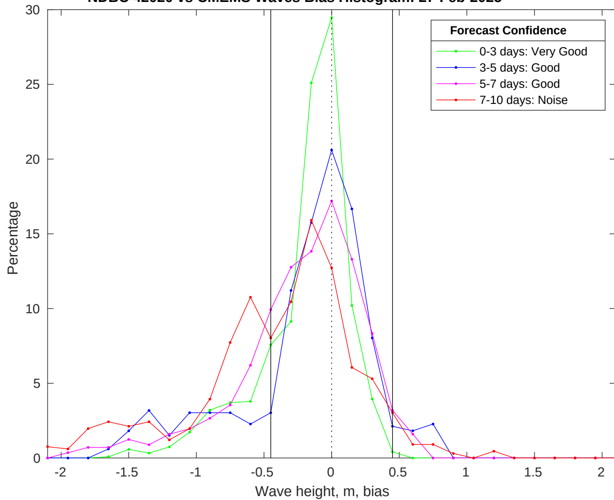
NDBC 42020 vs CMEMS Waves Bias Histogram: 27-Feb-2025
