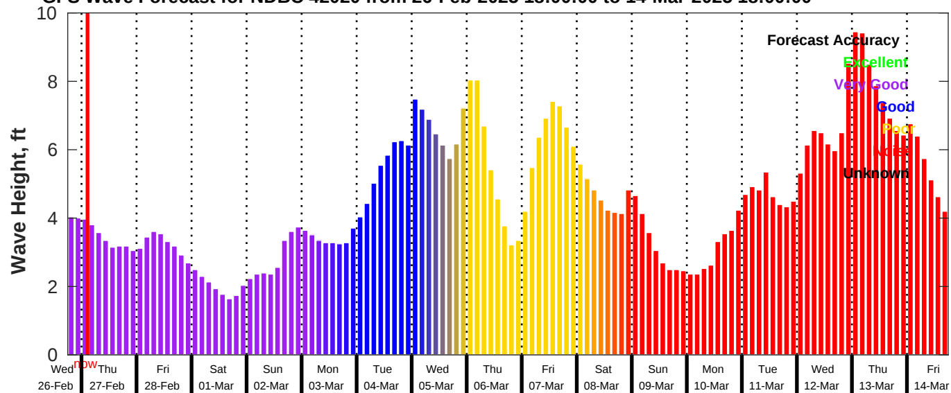
GFS Wave Forecast for NDBC 42020 from 26-Feb-2025 18:00:00 to 14-Mar-2025 18:00:00
