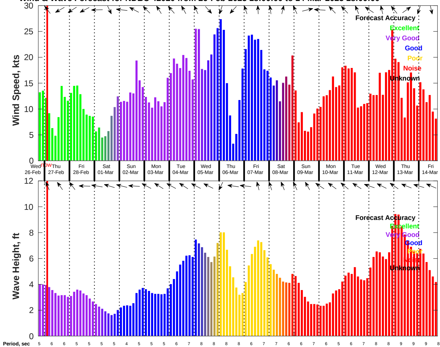
Wind & Wave Forecast for NDBC 42020 from 26-Feb-2025 18:00:00 to 14-Mar-2025 18:00:00
