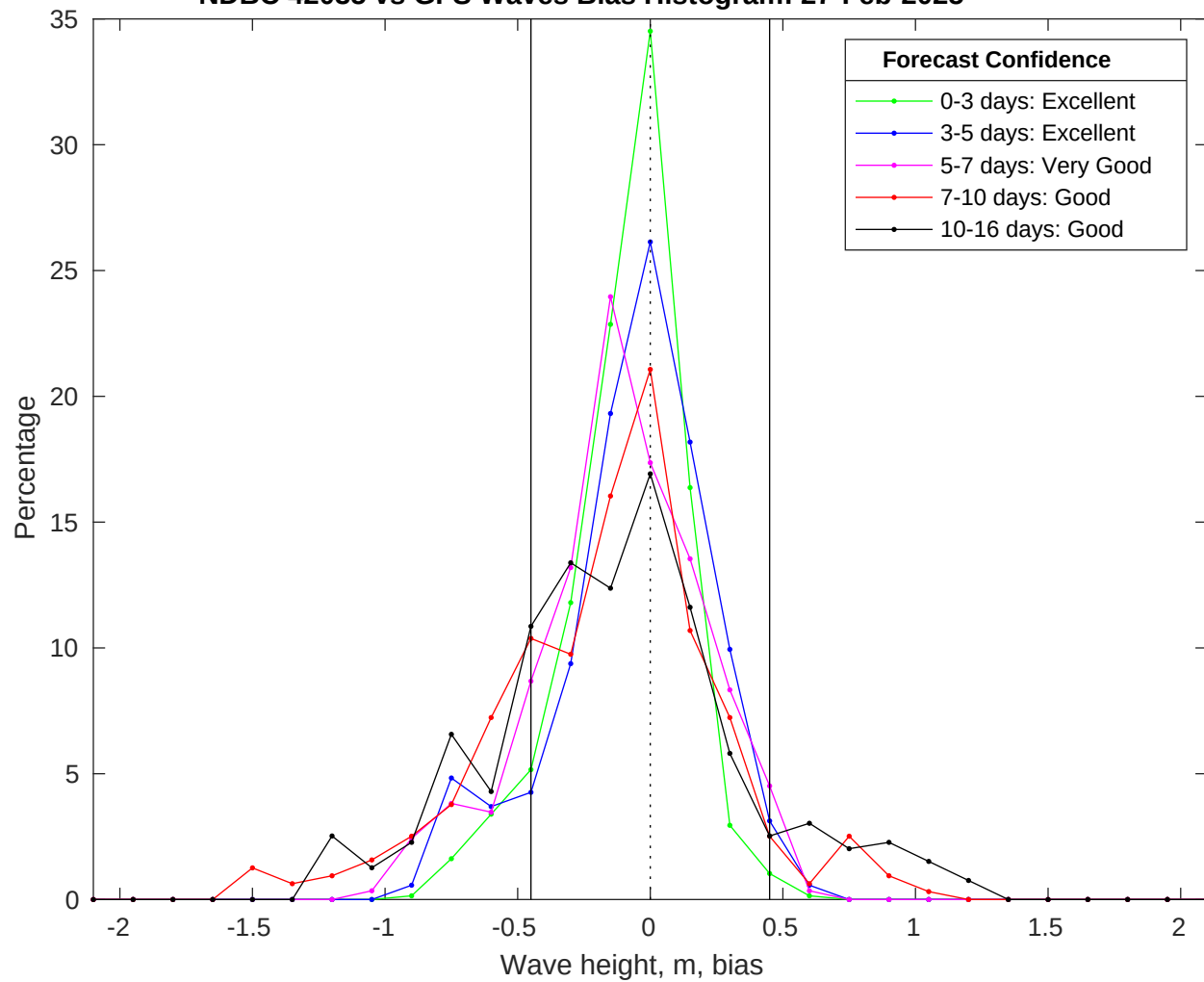
NDBC 42035 vs GFS Waves Bias Histogram: 27-Feb-2025
