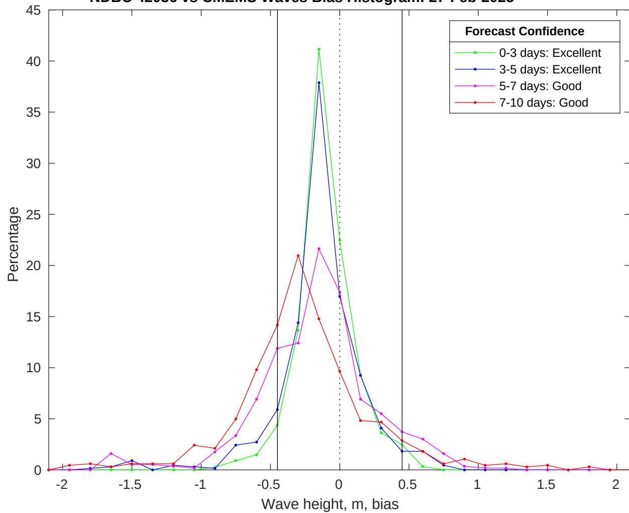
NDBC 42036 vs CMEMS Waves Bias Histogram: 27-Feb-2025
