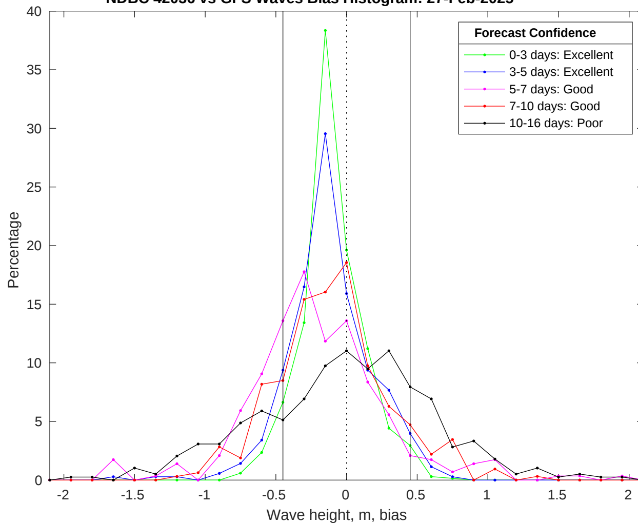
NDBC 42036 vs GFS Waves Bias Histogram: 27-Feb-2025
