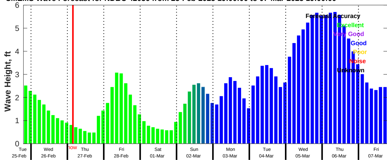
CMEMS Wave Forecast for NDBC 42036 from 25-Feb-2025 19:00:00 to 07-Mar-2025 19:00:00
