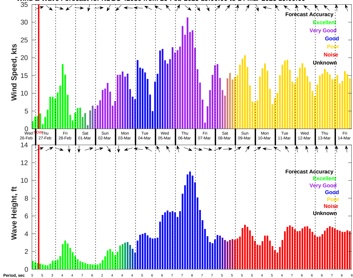
Wind & Wave Forecast for NDBC 42036 from 26-Feb-2025 19:00:00 to 14-Mar-2025 19:00:00
