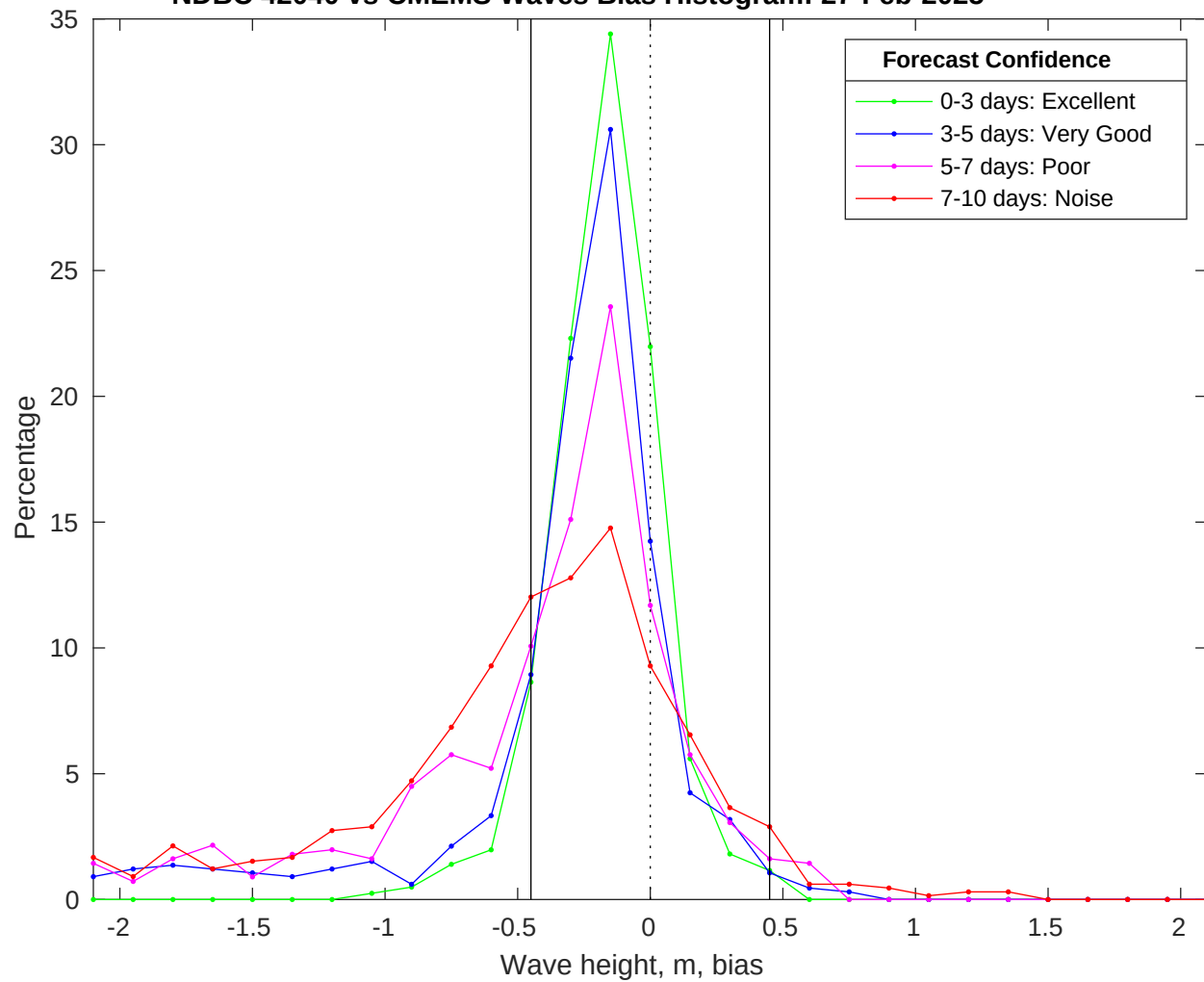
NDBC 42040 vs CMEMS Waves Bias Histogram: 27-Feb-2025
