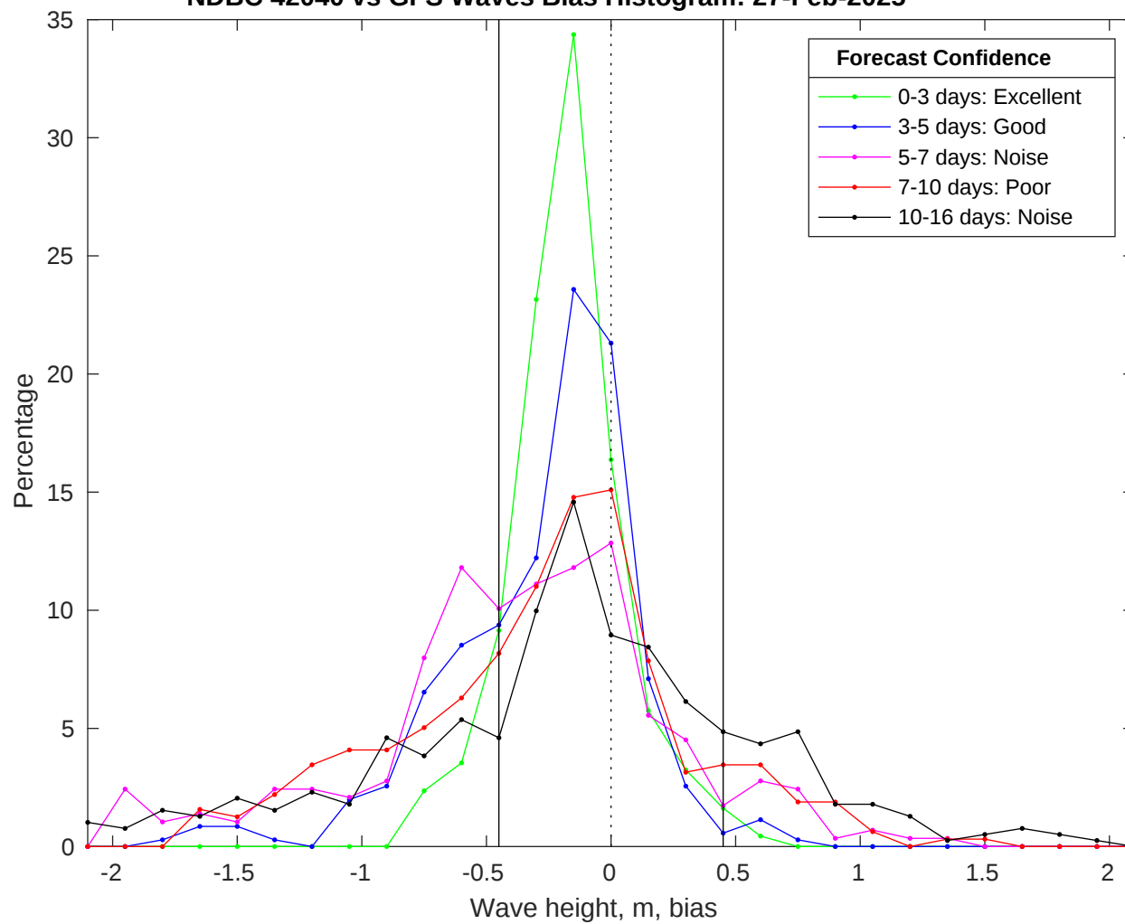
NDBC 42040 vs GFS Waves Bias Histogram: 27-Feb-2025
