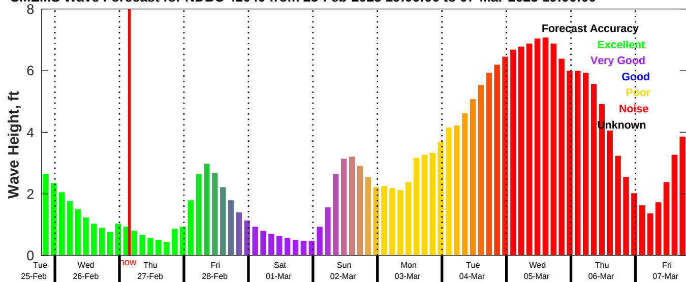
CMEMS Wave Forecast for NDBC 42040 from 25-Feb-2025 19:00:00 to 07-Mar-2025 19:00:00
