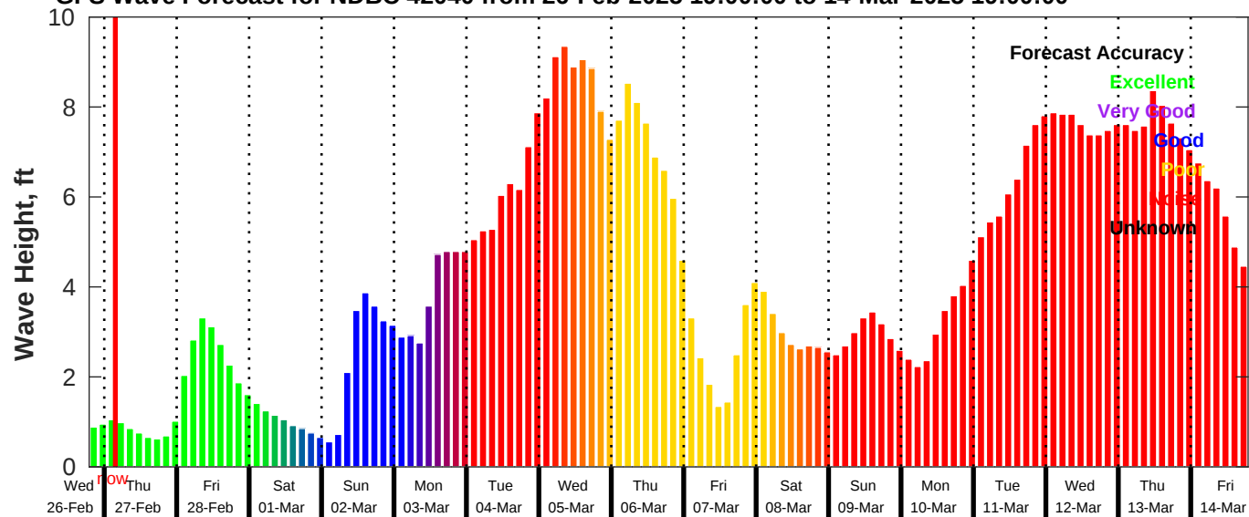
GFS Wave Forecast for NDBC 42040 from 26-Feb-2025 19:00:00 to 14-Mar-2025 19:00:00
