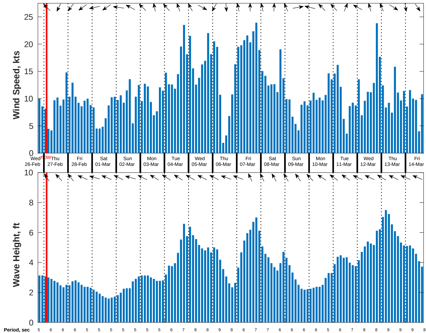
Wind & Wave Forecast for NDBC 42092 from 26-Feb-2025 18:00:00 to 14-Mar-2025 18:00:00
