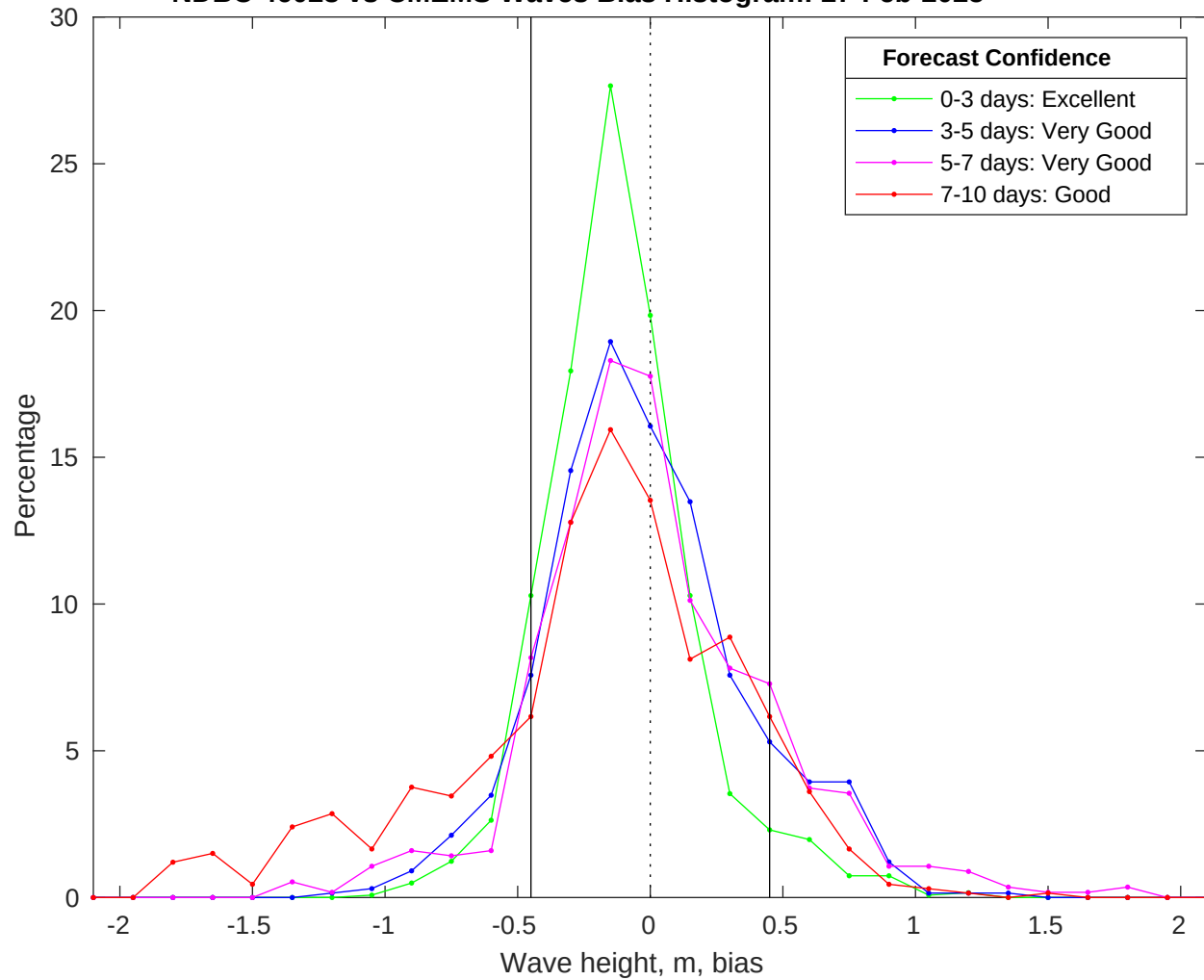
NDBC 46028 vs CMEMS Waves Bias Histogram: 27-Feb-2025
