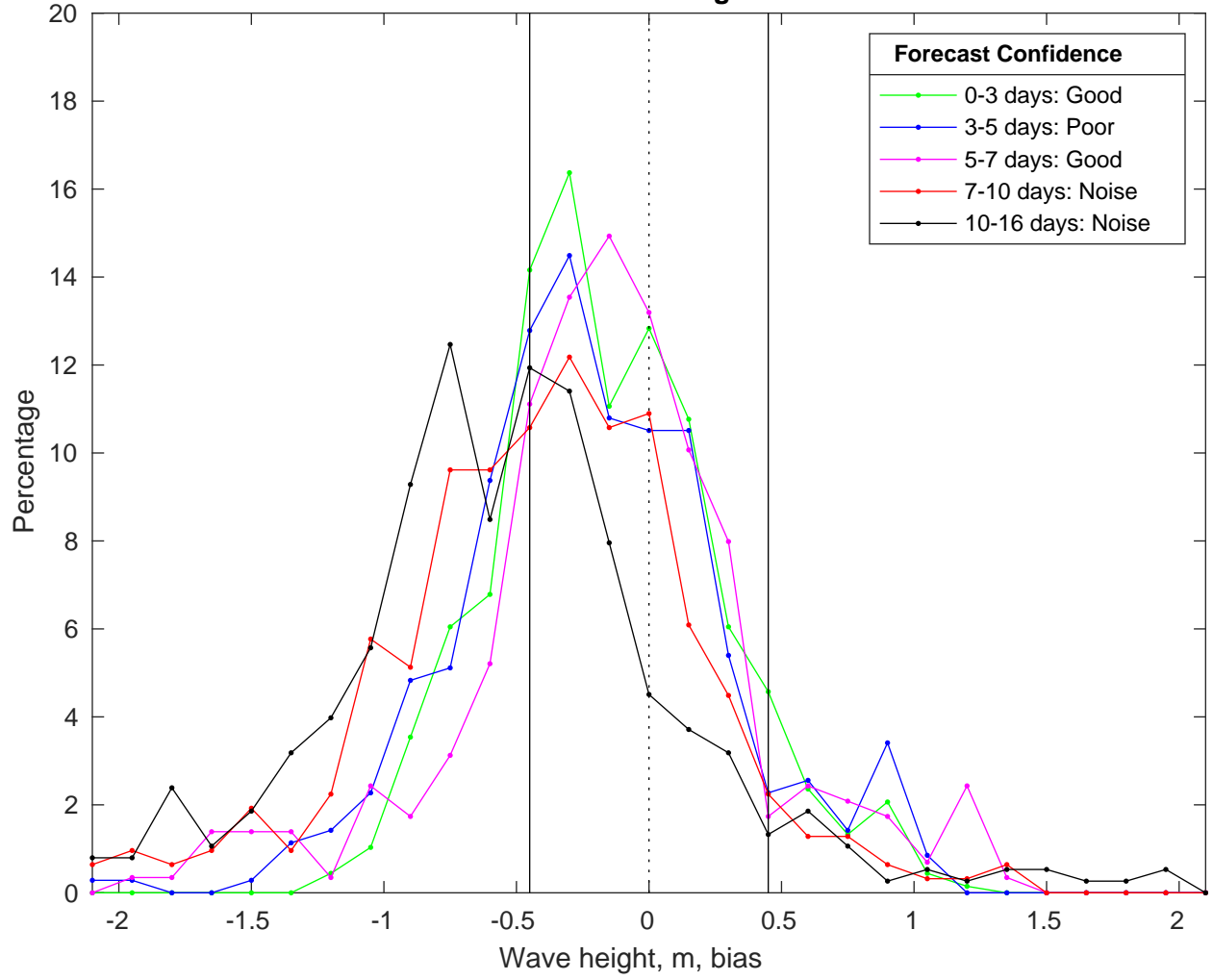
NDBC 46028 vs GFS Waves Bias Histogram: 27-Feb-2025
