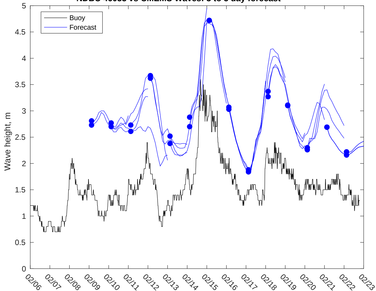
NDBC 46053 vs CMEMS Waves: 3 to 5 day forecast
