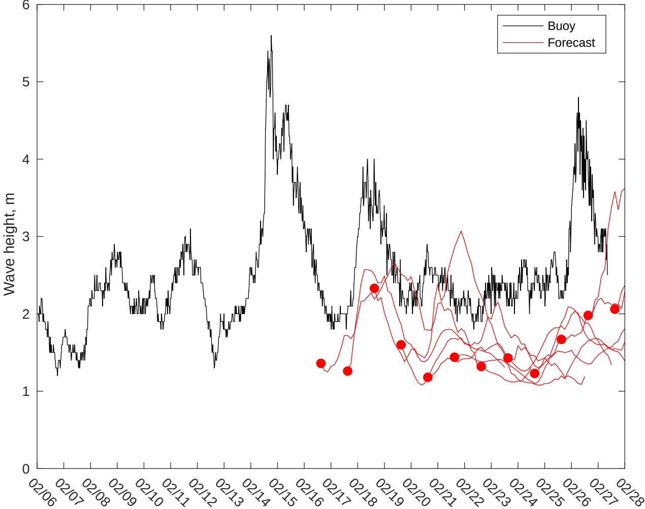
NDBC 46054 vs GFS Waves: 10 to 16 day forecast
