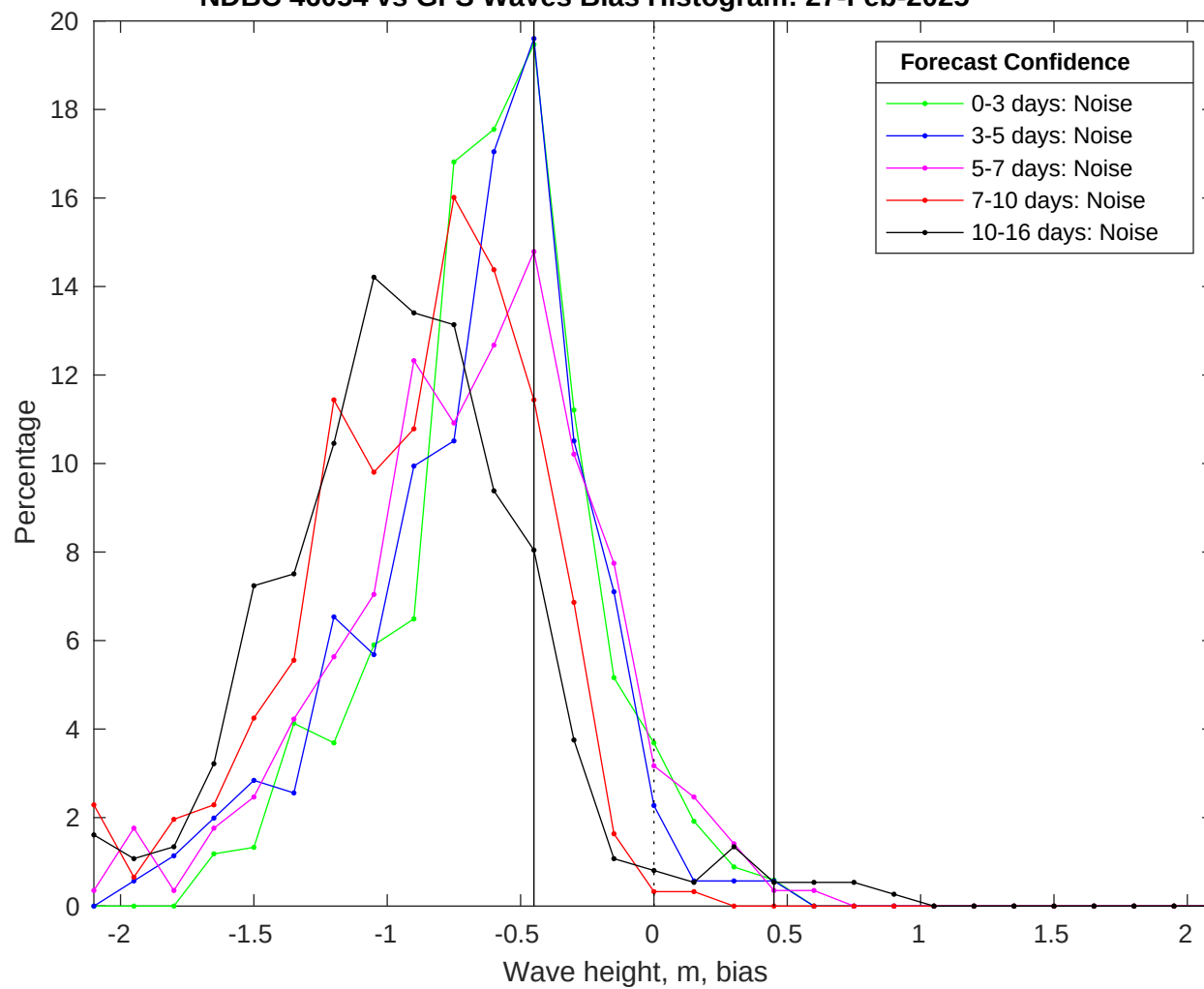
NDBC 46054 vs GFS Waves Bias Histogram: 27-Feb-2025
