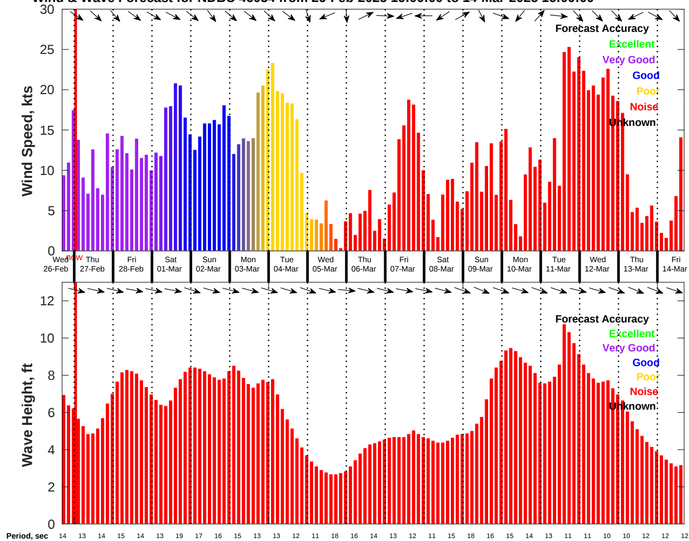
Wind & Wave Forecast for NDBC 46054 from 26-Feb-2025 16:00:00 to 14-Mar-2025 16:00:00
