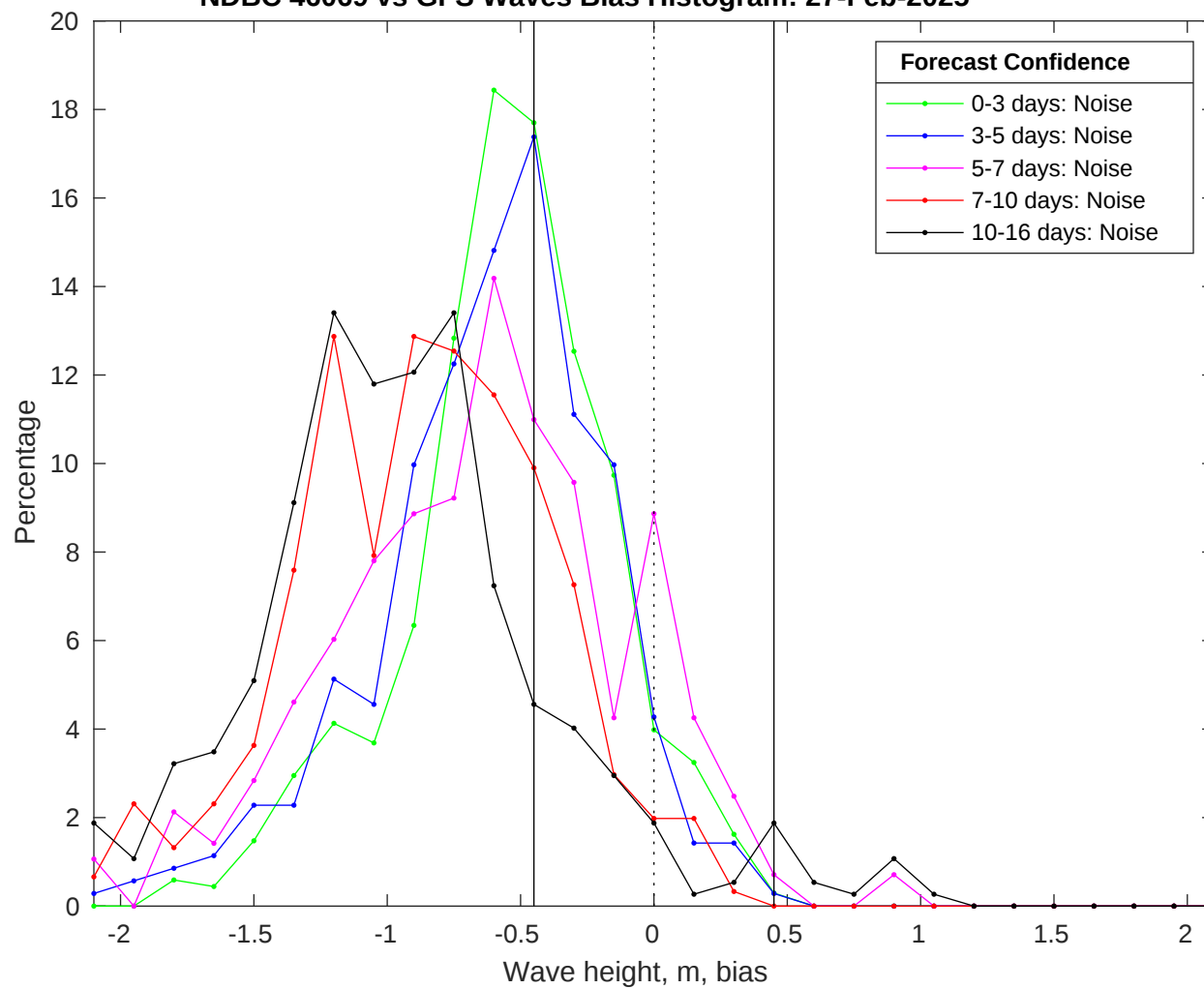
NDBC 46069 vs GFS Waves Bias Histogram: 27-Feb-2025
