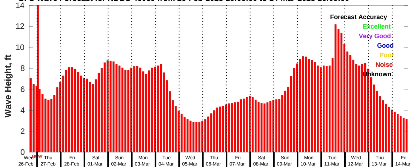
GFS Wave Forecast for NDBC 46069 from 26-Feb-2025 16:00:00 to 14-Mar-2025 16:00:00
