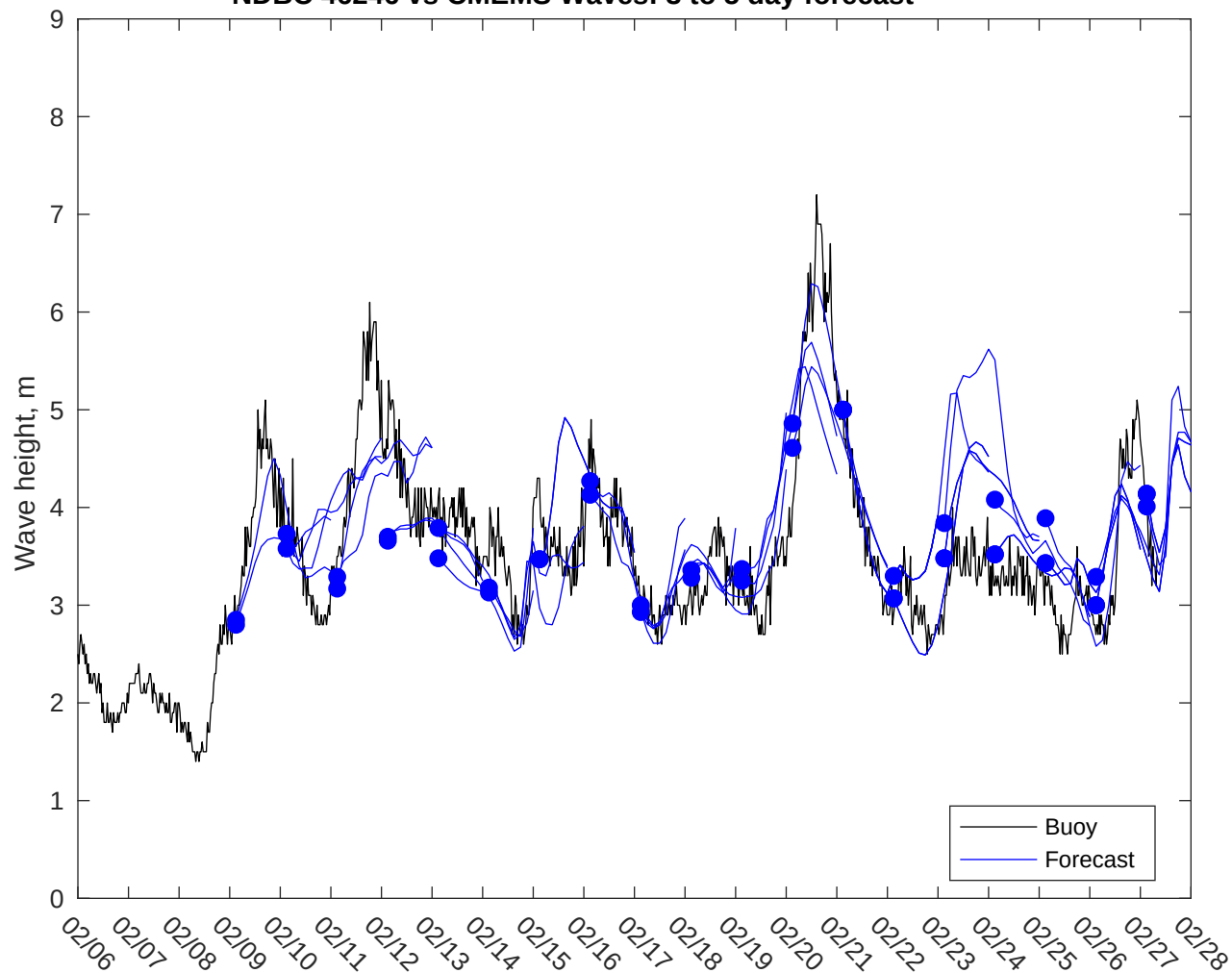
NDBC 46246 vs CMEMS Waves: 3 to 5 day forecast
