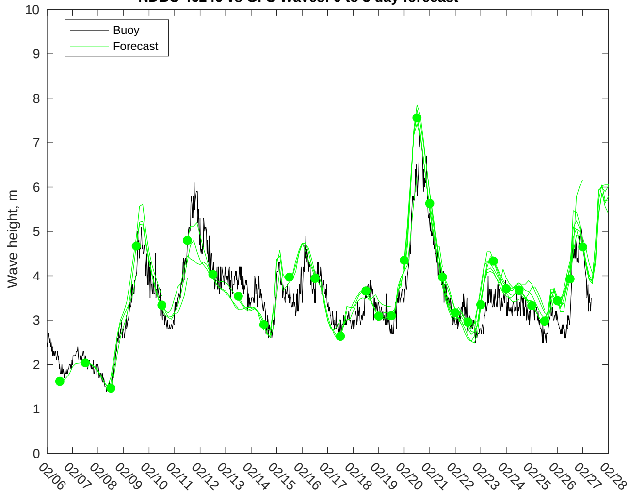
NDBC 46246 vs GFS Waves: 0 to 3 day forecast
