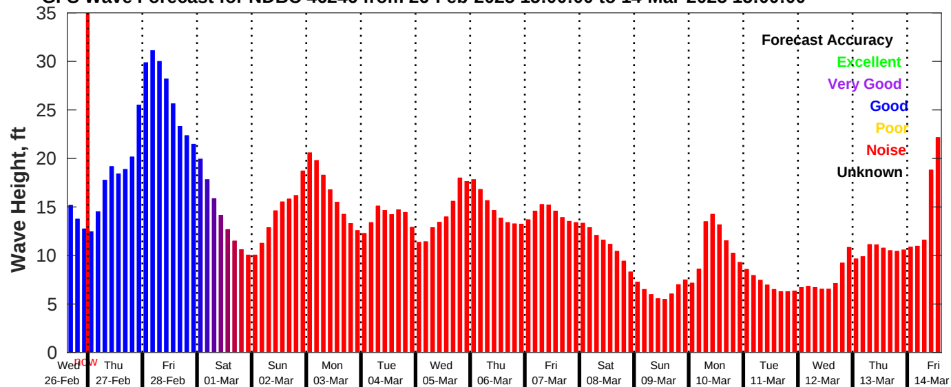
GFS Wave Forecast for NDBC 46246 from 26-Feb-2025 15:00:00 to 14-Mar-2025 15:00:00
