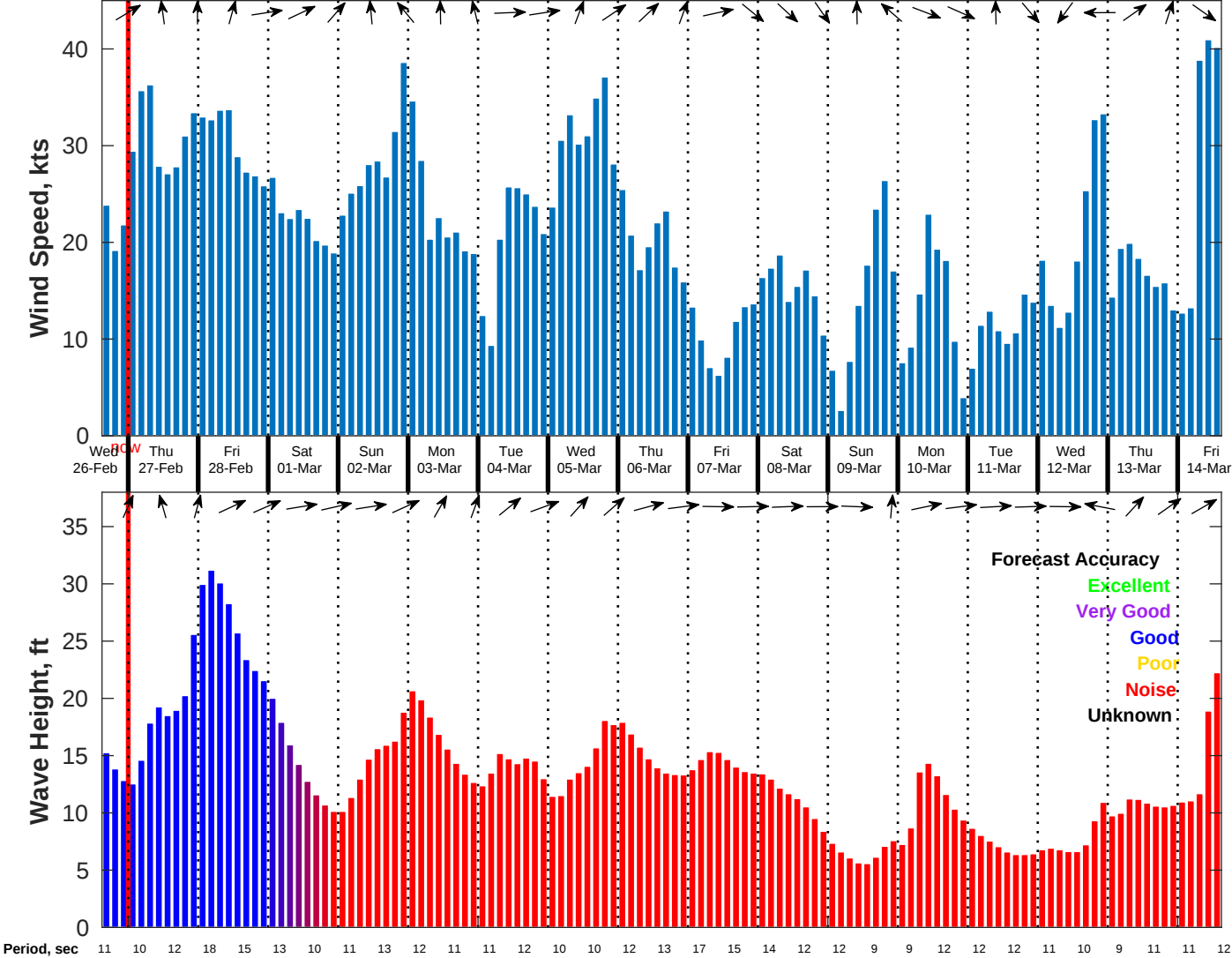
Wind & Wave Forecast for NDBC 46246 from 26-Feb-2025 15:00:00 to 14-Mar-2025 15:00:00
