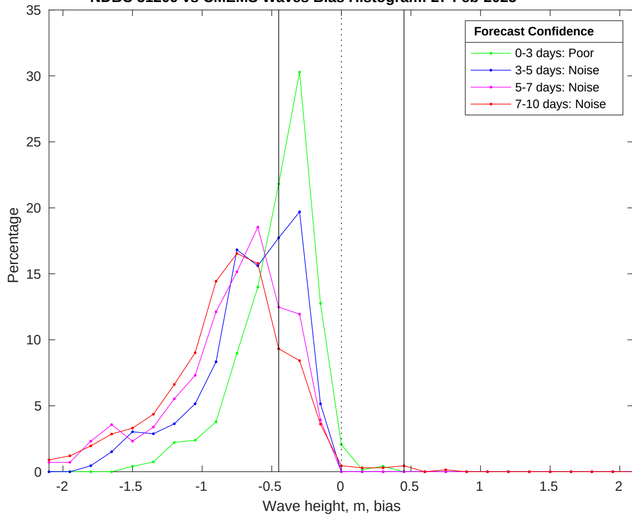
NDBC 51209 vs CMEMS Waves Bias Histogram: 27-Feb-2025
