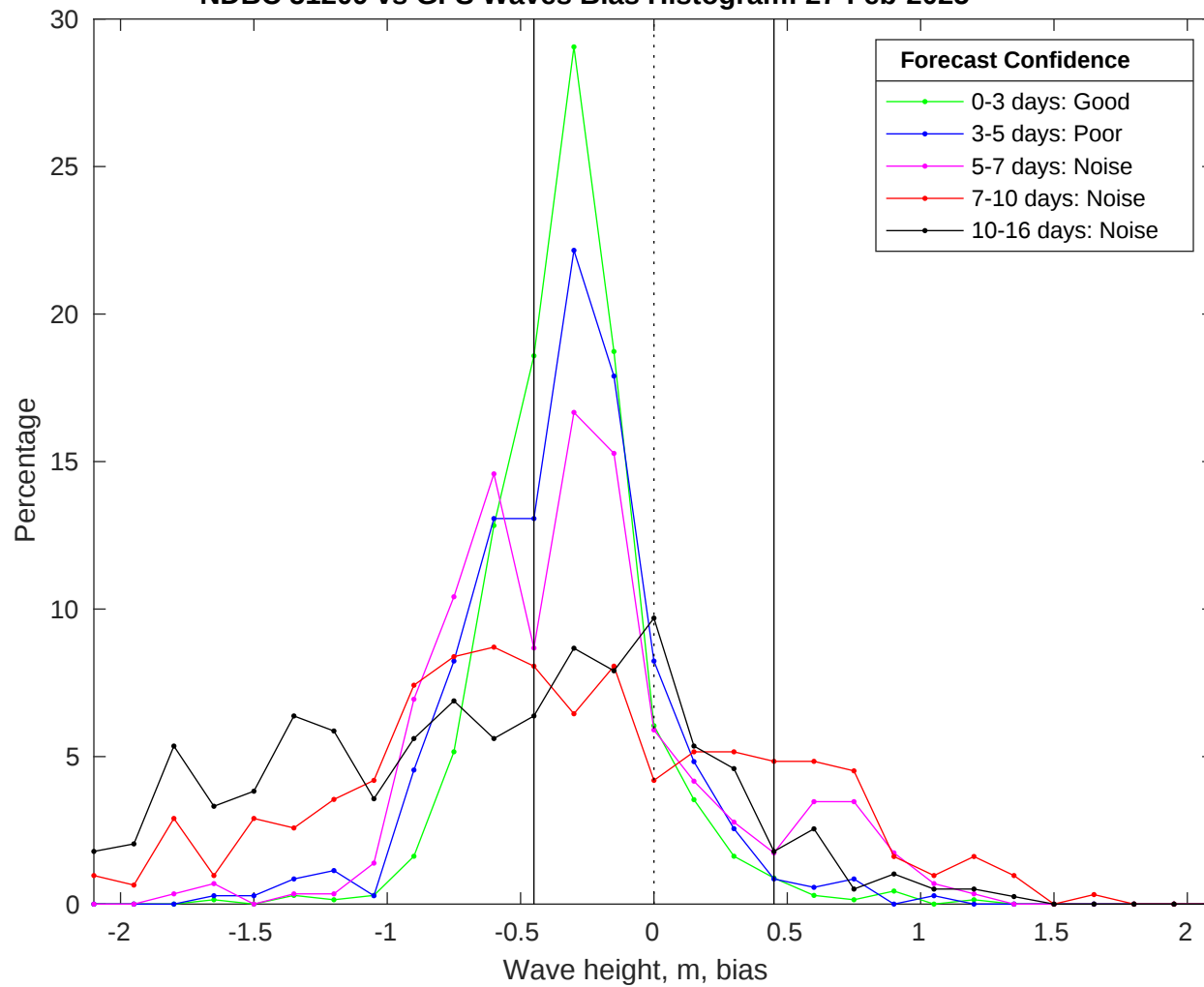
NDBC 51209 vs GFS Waves Bias Histogram: 27-Feb-2025
