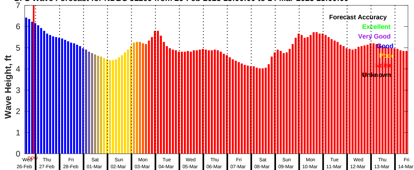
GFS Wave Forecast for NDBC 51209 from 26-Feb-2025 13:00:00 to 14-Mar-2025 13:00:00
