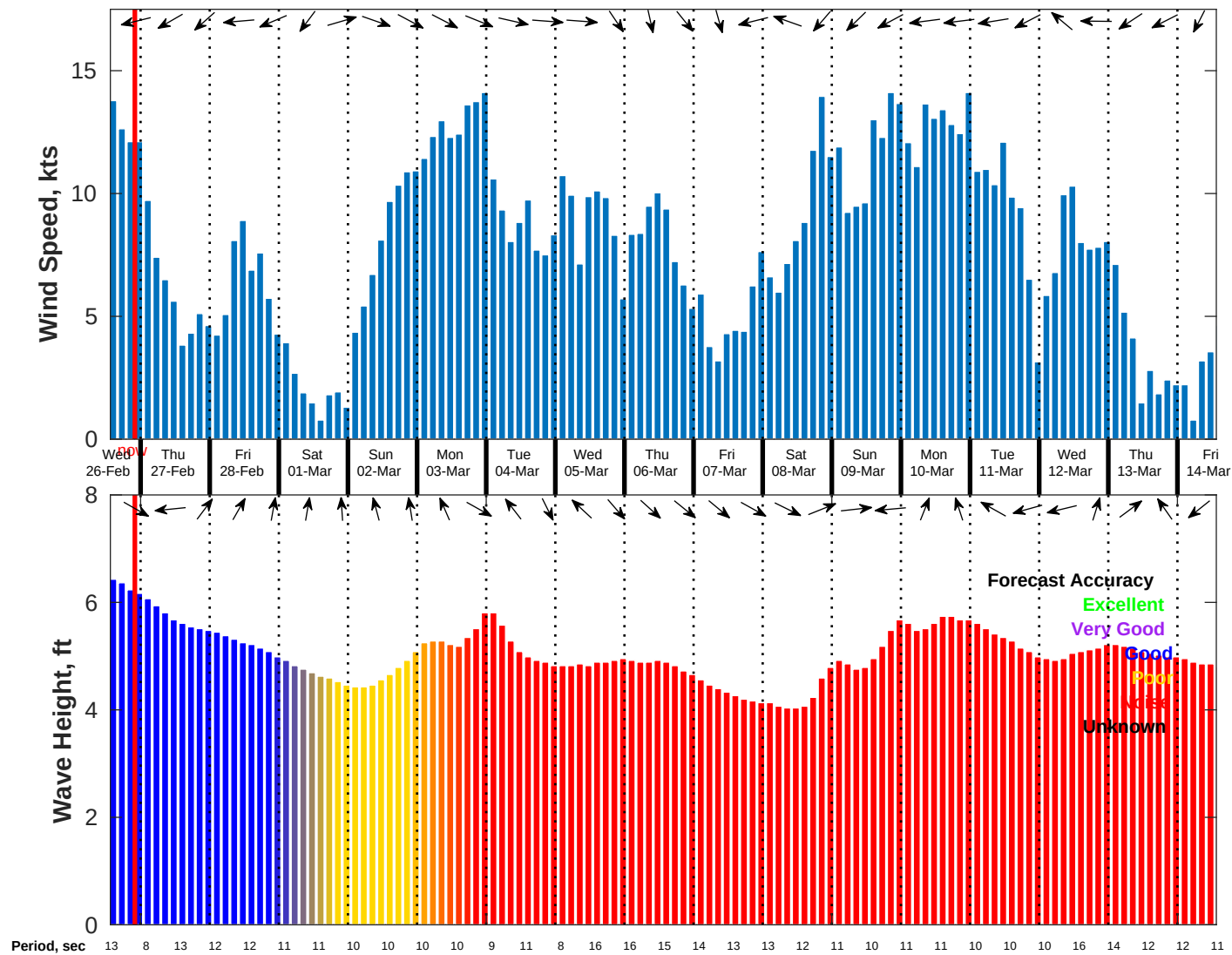
Wind & Wave Forecast for NDBC 51209 from 26-Feb-2025 13:00:00 to 14-Mar-2025 13:00:00
