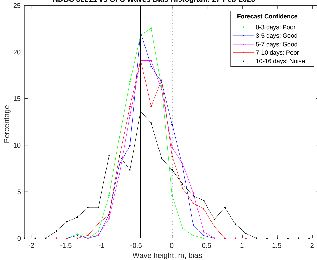
NDBC 52211 vs GFS Waves Bias Histogram: 27-Feb-2025
