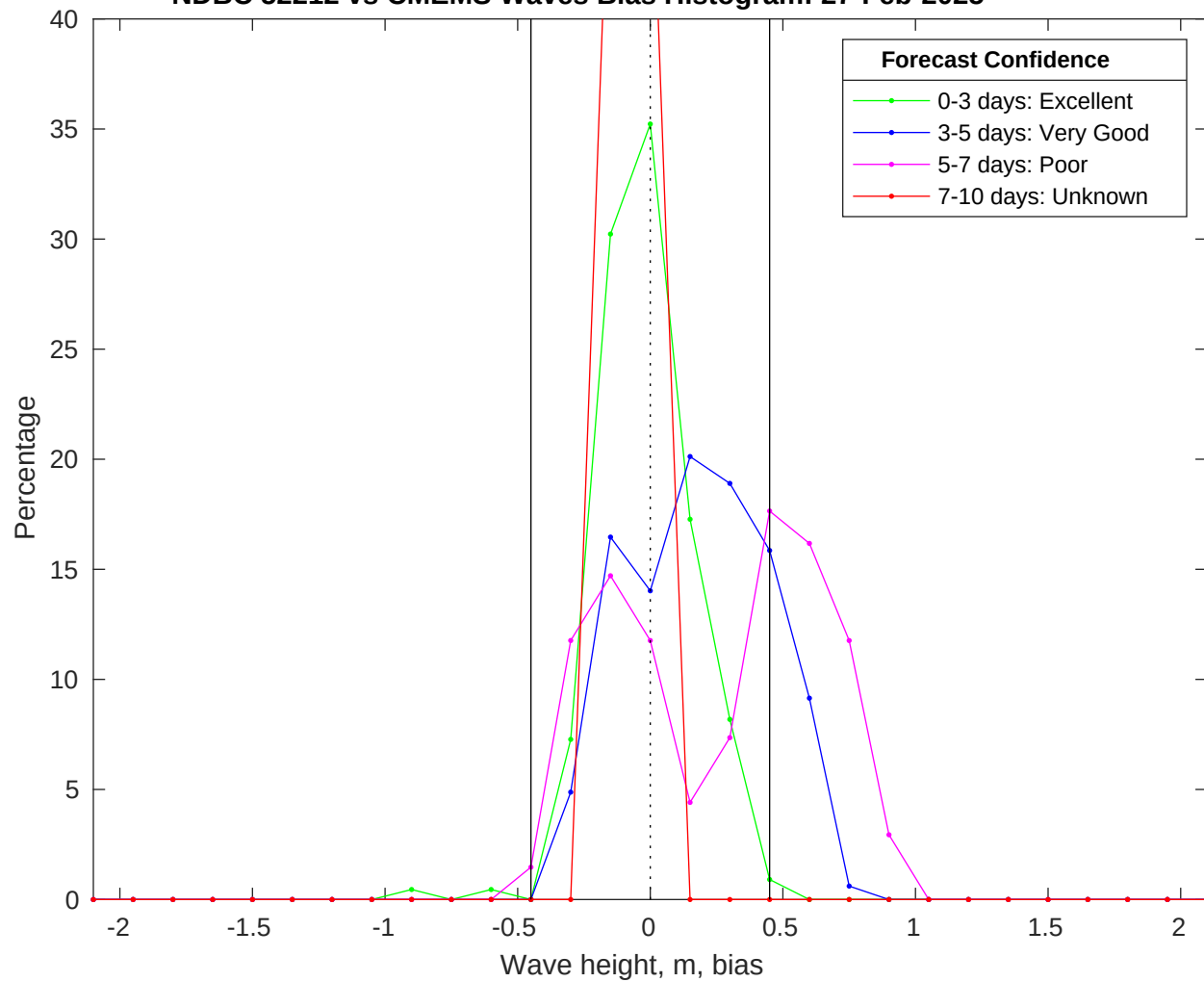
NDBC 52212 vs CMEMS Waves Bias Histogram: 27-Feb-2025
