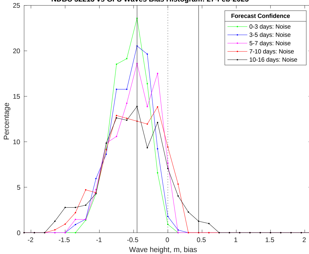
NDBC 52213 vs GFS Waves Bias Histogram: 27-Feb-2025
