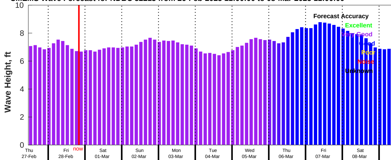
CMEMS Wave Forecast for NDBC 52213 from 26-Feb-2025 11:00:00 to 08-Mar-2025 11:00:00
