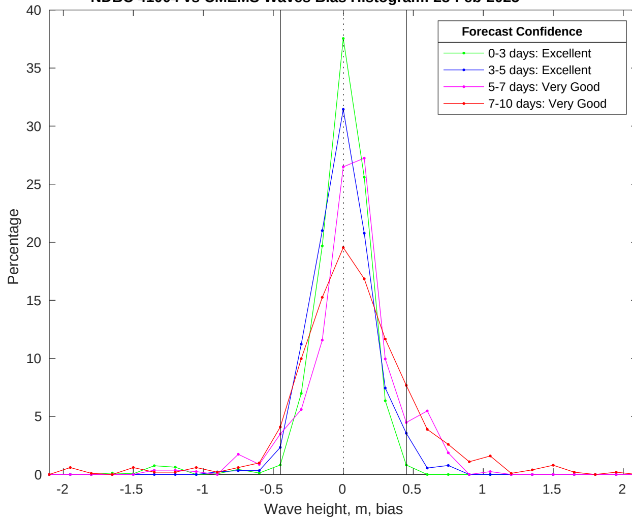
NDBC 41004 vs CMEMS Waves Bias Histogram: 28-Feb-2025
